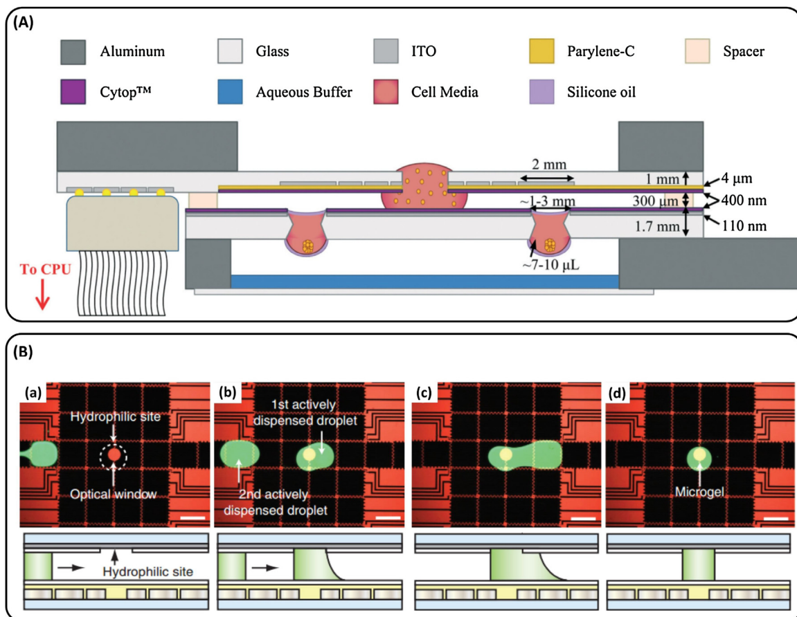
Fig. 9. Digital microfluidic chips for spheroid formation. (A) An HD-based digital \mu SFC. As shown in the figure, the platform design is complex and needs several materials such as Aluminum, Parylene-C, silicon oil, etc. as well as high resolution in fabrication (400 and 110 nm layers). A cell suspension is first introduced to the device inlet. Then, droplets are guided to the sites where the holes exist by the aid of capillary forces in order to form HDs and spheroids consequently. The humidified environment is provided by a buffer to prevent droplet evaporation for the long-term experiment. Reproduced with permission from [173]. (B) The process of droplet manipulation and anchoring in a digital microfluidic chip: (a) introducing the first droplet to the chip and guiding it to the hydrophilic site; (b) anchoring of the first droplet and introducing the second droplet to the first droplet; (c) the droplet moves across the hydrophilic site to facilitate the formation of a droplet similar to the hydrophilic pattern; (d) cross-linking leads to forming a solid microgel. Reproduced with permission from [178].
