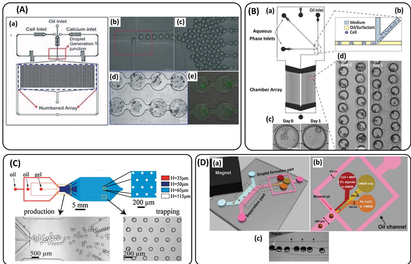
Fig. 3. (A) Single-emulsion (Gel/O) droplet generation chip for spheroid generation having sinusoidal anchoring array for (a) single cell type encapsulation; (b and c) T-junction for droplet formation and droplets entering the array before gelation; (d) Gelled cell-laden alginate spheroids; (e) Live cells stained with Calcein-AM. Reproduced with permission from [36]. (B) Single-emulsion (CS/O) spheroid formation device containing sinusoidal anchoring arrays. (a) Device overview showing the inlets and the anchoring array having 2000 droplet sites; (b) Droplet formation and cell encapsulation. (c and d) Brightfield images of cells encapsulated within droplets and trapped within the anchoring array (Reproduced with permission from [103]). (C) Single-emulsion (Gel/O) device using microwells to anchor cell-dispensed hydrogel droplets. (a) A schematic showing the oil and the hydrogel inlets and 2200 anchoring sites within the blue area; (b) Droplet production stage and the V-shaped trails for distributing the droplets over the anchoring sites. Reproduced with permission from [104]. (D) Another single-emulsion (Gel/O) chip producing droplets having magnetic particles on which magnetic force is exerted to deviate their pathway from the oil flow (pink) to the culture medium flow (blue). (a) Schematic depicting the overall view of the microfluidic chip; (b) The droplet generation section has four inlets: one dedicated to mineral oil and the others for \text{CaCl}_2 , culture medium and cell dispensed alginate hydrogel solved in culture medium; (c) A microscopic image of the separation channel. The magnet attracts the gelled droplets containing cells and magnetic nanoparticles to make them enter the culture medium from the oil. The broken line indicates the path line of a droplet. Reproduced with permission from [105]. (For interpretation of the references to colour in this figure legend, the reader is referred to the web version of this article.)
