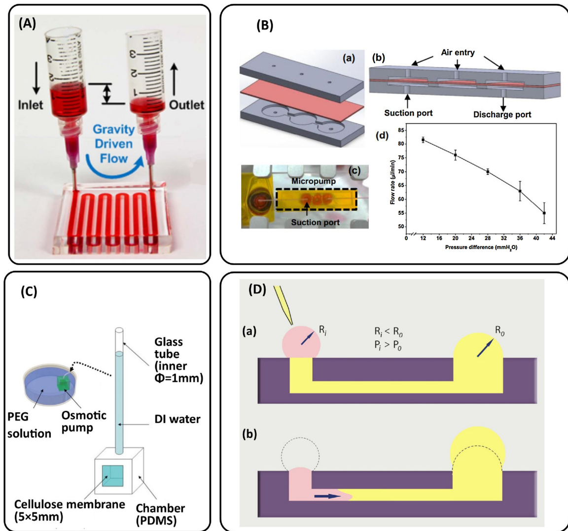
Fig. 14. Various methods for flow pumping in microfluidic chips. (A) Hydrostatic pressure drives flow through a \mu\text{SFC} . Reproduced with permission from [7]. (B) Peristaltic pump designed by Mousavi et al. [188]. (a) Schematic view of the micropump consisting of three layers which are two PDMS layers in the top and bottom of the device in addition to a diaphragm layer (red). By inducing low pressures in the air entry, flow is promoted from the suction port to the central chamber. Conversely, when applying high pressure in the air entry, the liquid in the chamber flows towards the discharge port; (b) cross-sectional view, showing the air and the liquid ports; (c) overall view; (d) the diagram of the pumping flow rate vs. pressure difference of the micropump. Reproduced with permission from [188]. (C) Schematic view of an osmotic pump designed by Park et al. comprised of water in a glass tube, a PDMS chamber containing water and a cellulose membrane [192]. The chamber is placed in a dish containing poly (ethylene glycol) solution in order to encourage liquid flow from the cellulose membrane to the dish. Reproduced with permission from [192]. (D) Passive pumping is facilitated by: (a) putting droplets at the inlet and the outlet channels having different volumes; (b) promotion of flow through the device from the smaller droplet to the larger one as a result of Laplace pressure difference caused by liquid surface tension. Redrawn after [194]. (For interpretation of the references to colour in this figure legend, the reader is referred to the web version of this article.)
