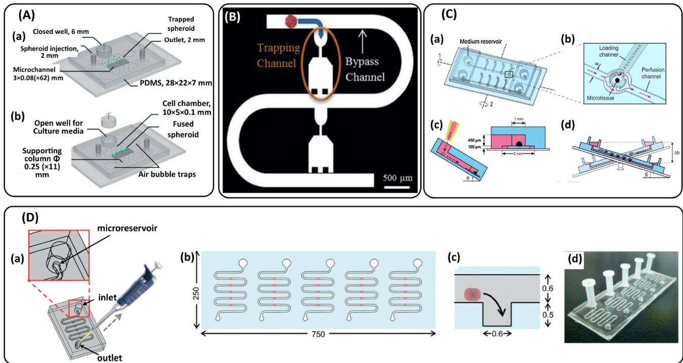
Fig. 8. The figure depicts various \mu SCCs. (A) A \mu SCC for culturing olfactory ensheathing cell spheroids. (a) This device consists of two inlets: one large well (6 mm) for culture medium and a smaller one (2 mm) for spheroid injection. Parallel microchannels, 80 \mu m in width for spheroid trapping, are embedded within the device through which the culture medium passes and feeds the spheroids; (b) the device also integrates lateral chambers for trapping unwanted air bubbles entering the device. Reproduced with permission from [87]. (B) The microchannels are designed using the hydraulic-electric analogy in which the trapping channel has less flow resistance than the bypass channel before spheroid trapping. Reproduced with permission from [8]. (C) A hydrostatic pressure-driven \mu SCC containing two units each having one perfusion and four loading microchannels. (a) Medium reservoirs are situated at both ends of each perfusion microchannel; (b) the spheroid culture chamber is placed at the intersection of the loading and the perfusion microchannel; (c) to load spheroids, the device is slanted with respect to axis No. 1 in figure (a); (d) After spheroid loading into the chambers, flow is created by periodic tilting of the device around axis No. 2 to obtain hydrostatic pressure difference between the inlet and outlet. Reproduced with permission from [89]. (D) A \mu SCC consisting of five parallel sinuous microchannels each of which contains five microwells for sedimentation trapping of the loaded microtissues or spheroids. (a) Loading microtissues or spheroids into the chip by a micropipette; (b) The microchip with five independent microchannels each has five equally-spaced microwell traps (red); (c) side view of the microtissue in the microchannel which is reaching the microwell trap; (d) the microchip made of PDMS with five inlet reservoirs. Reproduced with permission from [139]. (For interpretation of the references to colour in this figure legend, the reader is referred to the web version of this article.)
