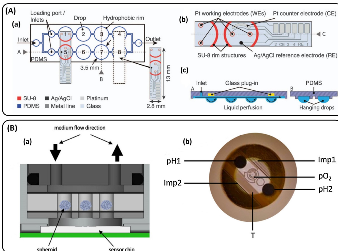
Fig. 17. (A) An HD-based \mu SFC integrated with a biosensor for lactate and glucose measurements; (a) schematic view of the device having 8 HD sites of 3.5 mm diameter and the orientation of the biosensor on the chip; (b) the electrode-based biosensor is displayed. The sensor consists of four working platinum electrodes, one platinum counter electrode and an Ag/AgCl reference electrode; (c) the cross-section views A and B clarify the flow in the microchannels and the yellow glass plug-ins on which the sensors are deposited. Reproduced with permission from [207]; (B) A cross-sectional view of the \mu SCC (a) and the sensor chip (b) designed by Alexander et al. [209]; (a) It consists of a fluidic channel in the top, three 1 mm diameter microwells containing the spheroids and a sensor microchip in the bottom of the porous membranes; (b) the sensor chip measures the pH of the microenvironment (pH1 and pH2 sensors), oxygen uptake rate by the cells ( pO_2 amperometric sensor), temperature (T) and electrical impedance (Imp1 and Imp2) by the electrodes shown in the figure. Reproduced with permission from [209]. (For interpretation of the references to colour in this figure legend, the reader is referred to the web version of this article.)
