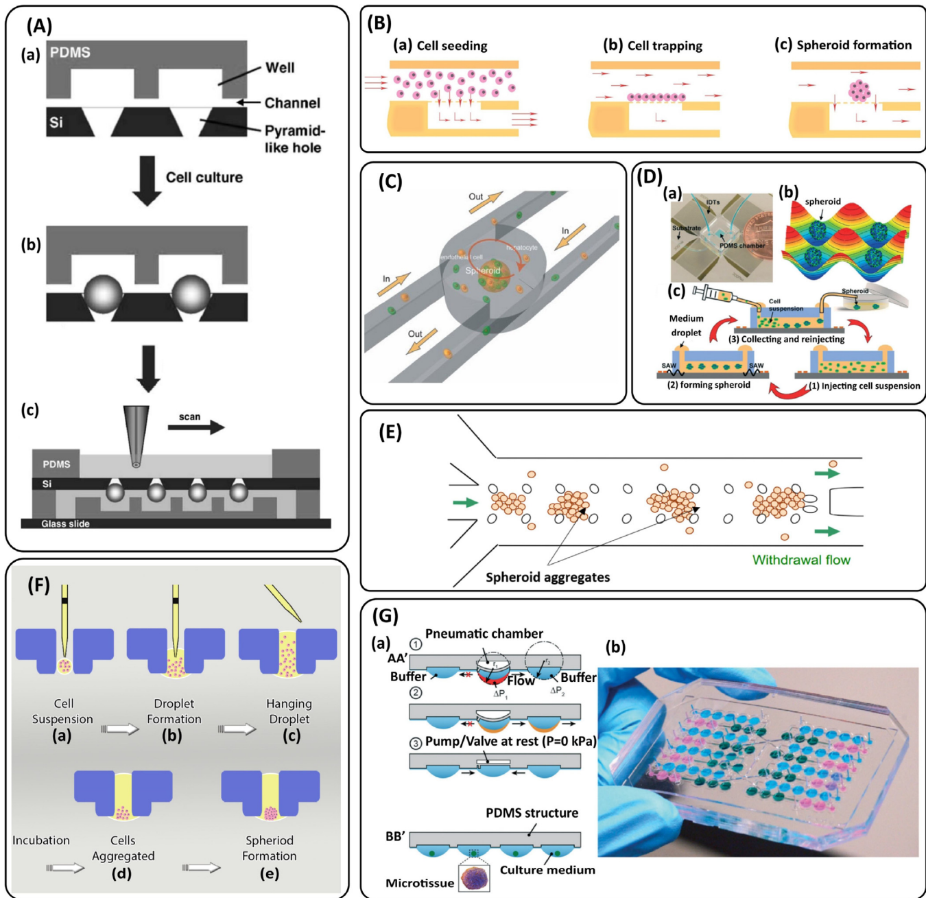
Fig. 7. Other types of \mu SFCs: (A) A \mu SFC compatible with SECM due to silicon pyramid-like holes. (a) The cross-section of the microchip is depicted and its layers are shown; (b) The figure shows the microchip after spheroids have been formed in the structures resembling HDs; (c) The SECM measurement was done on the microchip while it was inverted on a glass slide to avoid spilling of the measurement liquid. Reproduced with permission from [151]. (B) Cell trapping behind a porous membrane for spheroid formation, facilitated by the flow of the cell suspension through the membrane. The spheroid formation is carried out by: (a) cell seeding, (b) cell trapping behind the porous membrane and (c) cell aggregation. (C) Microrotational flow in a microchamber having two inlets and outlets embedded in a three-layered \mu SFC. The inlet and outlet channels are tangential to the cylinder in the middle layer and the upper layer, respectively, to promote rotational flow. Reproduced with permission from [152]. (D) Spheroid formation by the aid of 3D acoustic tweezers. (a) The overall view of the microchip is shown; (b) Diagram of Gor'kov potential field inside the cavity. The balance among the acoustic radiation force, microstreaming drag force, gravity and buoyant force aggregated the Cells; (c) First, the cell suspension is injected. Then, spheroids are formed in the microchannel where the potential field exists; the generated spheroids are then placed in a Petri dish. Reproduced with permission from [10]. (E) Cells are entered through the central inlet channel and trapped in the central chamber to form spheroids. The chamber is separated from the surrounding flow, which comes through the side inlets, by micropillars which are located close to each other. Reproduced with permission from [153]. (F) HD spheroid formation in an HD plate: (a) introduction of the cell suspension within the holes; (b) formation of the droplet by the capillary forces, (c) creation of an HD, (d) cell aggregation, (e) spheroid formation after one day. Redrawn after [54]. (G) an HD based \mu SFC. (a) The figure depicts (1) the pneumatic chamber is pressurized to create a flow from the central HD to the right HD (2). (3) The left valve, which prevented backflow, is now open while the pneumatic chamber is unpressurized. Fig. 4 shows the spheroids in the HDs; (b) an image of the HD based \mu SFC which is colored by food dyes. Reproduced with permission from [154].
