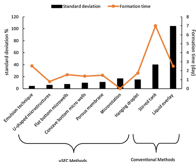
Fig. 10. The figure shows spheroid diameter standard deviation (the black columns) and formation time (the orange line) collected from a myriad of previous studies. The data belong to microfluidic and conventional methods for spheroid formation, displaying microfluidics' superior advantages in forming spheroids with a shorter time and also size uniformity. The SD extends from 4% for the emulsion technique to 16.6% for the microrotational flow \mu SFC. The formation time also differs significantly from the stirred tank method and \mu SFCs. (For interpretation of the references to colour in this figure legend, the reader is referred to the web version of this article.)
