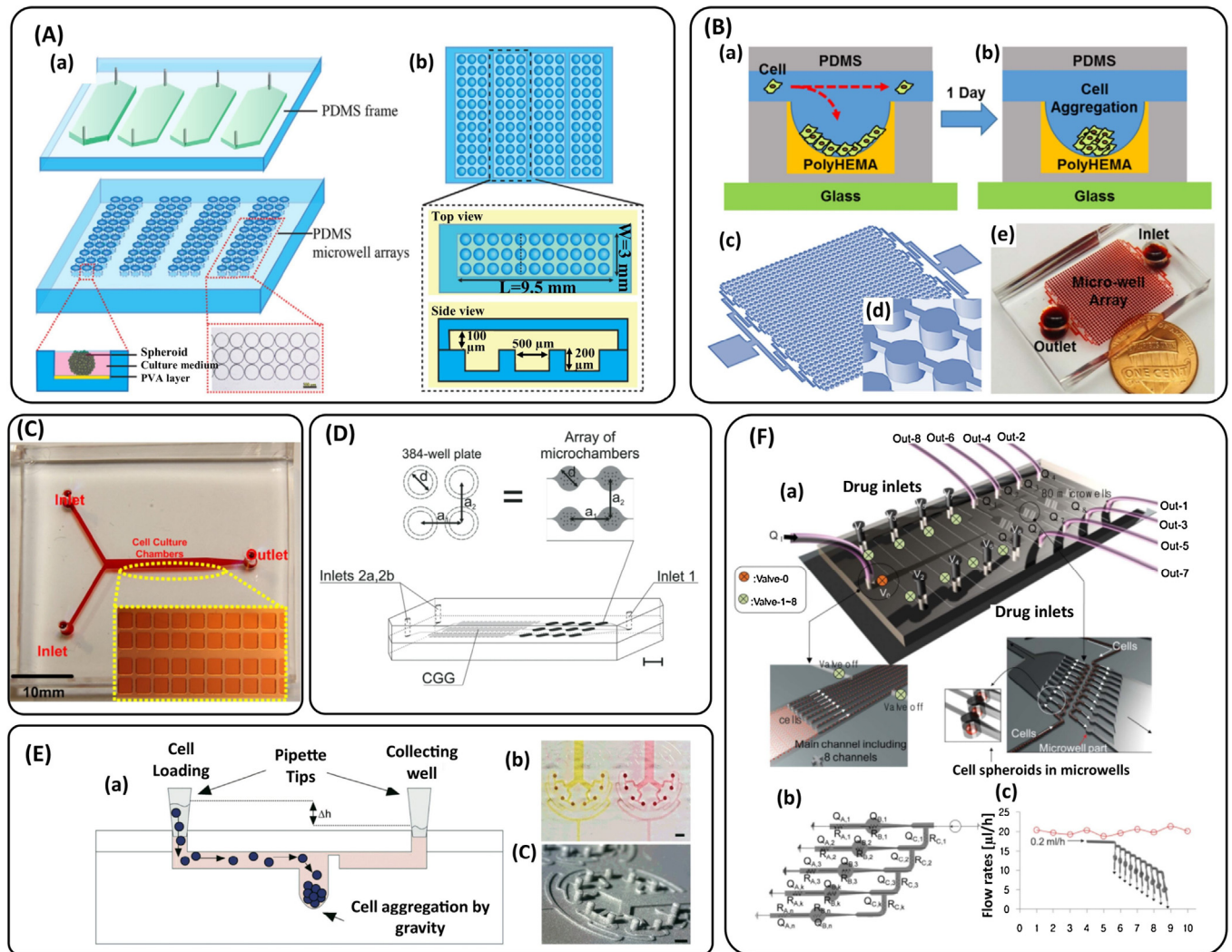
Fig. 6. Parts A to D depict microwell-based \mu SFCs in which each microchannel feeds several spheroids. In the parts E and F each main microchannel branches into several microchannels which individually feed each microwell. (A) A graphic demonstration of a microchip for MTS formation and drug screening. (a) Each microchannel feeds a 3 \times 11 configuration of microwells. The formation of a cell spheroid in a microwell displayed at the bottom left, and a micrograph of the microwell-array of the chip is shown at the bottom right; (b) Top and side visions of the microchip. Reproduced with permission from [134]. (B) A microwell-based \mu SFC for evaluating the efficacy of Photo Dynamic Therapy on tumor spheroids. (a) Graphical representation of cells trapping in a microwell; (b) Schematic of cell aggregation after 1 day; (c and d) The structure of the 3D microfluidic chip; (e) The fabricated chip that has 1024 microwells within a main area of 2 cm by 2 cm. Reproduced with permission from [13]. (C) Photographs of a two-layered \mu SFC, and the magnified view of the square spheroid culture microwells in the inset. Reproduced with permission from [96]. (D) A \mu SFC integrated with a CGG to facilitate high-throughput drug tests. Each drug is delivered to three microchambers in series, each containing 14 microwells. The distance between microchambers was designed such that the \mu SFC is compatible with conventional plate readers. Reproduced with permission from [6]. (E) A microwell-based \mu SFC having (a) Cells are trapped within each microwell due to the difference between the inlet and outlet microchannel heights; (b) Top-view of two microchannels filling with color food dyes (yellow and red). The length of the microchannels delivering cell suspension to each microwell is equal to facilitate uniform-sized spheroid formation; (c) The microchip's mold made of epoxy. Reproduced with permission from [39]. (F) A microwell-based \mu SFC designed using the hydraulic-electric analogy to facilitate spheroid culture of the same cell numbers in all the microwells. (a) It contains one inlet for cell seeding, eight inlets for drug perfusion and eight outlets; (b) Plane representation of the microchannel network in which the flow rates are adjusted by the hydrodynamic resistance of the microchannels; (c) The uniform flow rates in each microchannel estimated by hydrodynamic simulation. Reproduced with permission from [88]. (For interpretation of the references to colour in this figure legend, the reader is referred to the web version of this article.)
