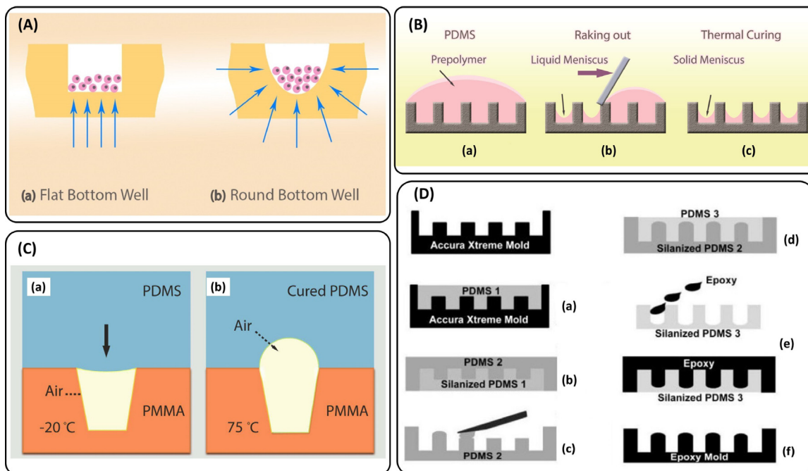
Fig. 13. (A) Illustration of the microforces acting on cells in a (a) flat-bottomed and (b) concave-bottomed microwell. Figures B to D depict fabrication methods to generate concave-bottomed microwells for spheroid formation: (B) creating concave-bottomed microwells using PDMS prepolymer by: (a) pouring the PDMS prepolymer on the microwells; (b) raking out the liquid meniscus and (c) thermal curing for PDMS solidification. Redrawn after [40]. (C) Using air expansion to induce concave shape on PDMS slab: (a) air is trapped in the microwell due to the high viscosity of cold PDMS; (b) during baking of PDMS, the air expands and pushes the PDMS upward. After baking, the PDMS slab is peeled off and used. Redrawn after [125]. (D) This method utilized silanization treatment to enable multi-casting of PDMS. All PDMS curing took place at 60° C for 2 h. (a) Mold is filled with PDMS and cured. (b) After silanization a second PDMS is produced and cured. (c) A little drop of PDMS is added on every well to round it and cured. (d) After silanization a 3rd PDMS cast is produced and cured. (e) After silanization the PDMS mold is filled with the epoxy (Weidling C) and cured at 40° C for 24 h. (f) Final epoxy mold with round bottom wells. Reproduced with permission from [39].
