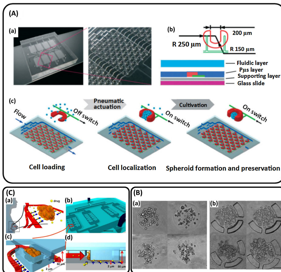
Fig. 4. U-shaped microstructures in \mu SFCs: (A) A pneumatically actuated \mu SFC containing U-shaped microstructure arrays. It contains eight chambers for high-throughput cell trapping and spheroid formation. (a) The two images depict the microchip fabricated out of PDMS; (b) Top and sectional view of one of the U-shaped microstructures comprised of three layers; (c) Schematic diagrams of high-throughput cell loading and localization within the chip. Reproduced with permission from [128]. (B) Permanent U-shaped microstructures. (a) The configuration of the alginate encapsulated beads instantly after droplet formation in a Petri dish; (b) This figure depicts the droplets four days after being trapped in the microstructure for spheroid formation. The gaps between the microsieves enable proper diffusional nutrient and gas exchange. Reproduced with permission from [18]. (C) A \mu SFC containing permanent U-shaped microstructures. (a) A representation of an in-vivo tumor provided by drug molecules from blood vessels; (b) The microchip constructed by PDMS/glass slide; (c and d) the flow of culture medium towards the microstructure pushes the cells inside. Drug, nutrient and waste molecules are perfused to the trapped cells with the flow through the 2 \mu m gap. Reproduced with permission from [121].
